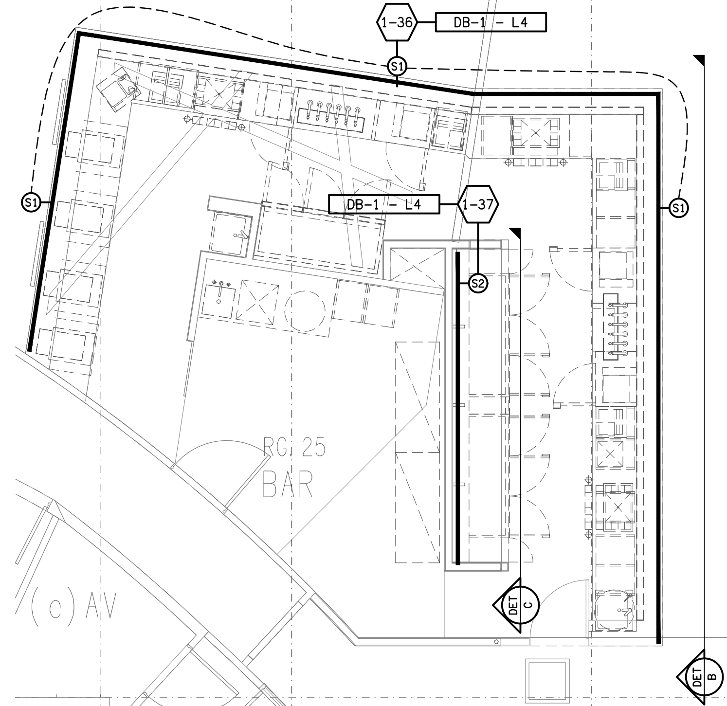
DETAIL A SPORTS BAR LIGHTING PLAN SCALE 1: 50
